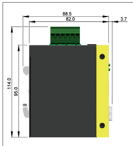
Din-Rail Mount Dimension
