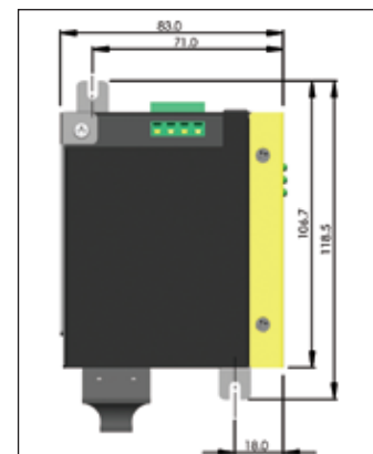
Panel & Wall Mount Dimension
