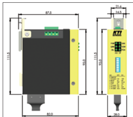
Din-Rail Mount Dimension
